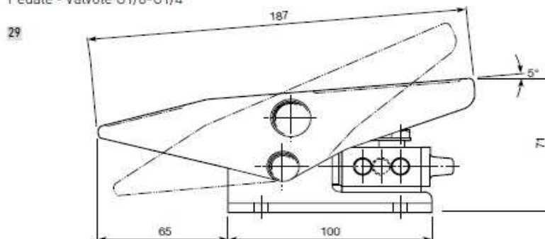
Pedale - valvole G1/8-G1/4
