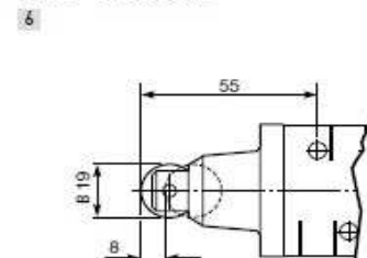
Rullo - valvole G1/4
