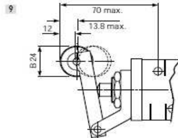
Leva a rulli - valvole G1/4
