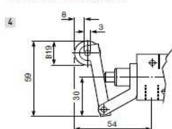
Leva a rulli - valvole G1/8
