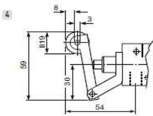
Leva a rulli - valvole G1/8" Roller lever - G1/8" valves
