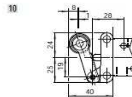
Leva a rulli (serv.pesante) G1/4" Roller lever Heavy Duty - G1/4"
