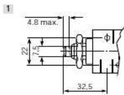
Pulsante - valvole G1/8" Button - G1/8" valves
