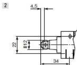
Leva a rulli sensibile- valvole G1/8" Sensitive roller lever - G1/8" valves
