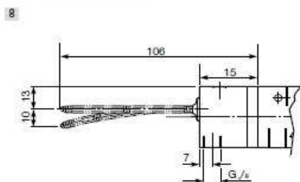
Antenna - valvole G1/8" Antenna - G1/8" valves
