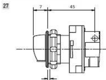
Manopola girevole - G1/8" Rotary knob - G1/8"
