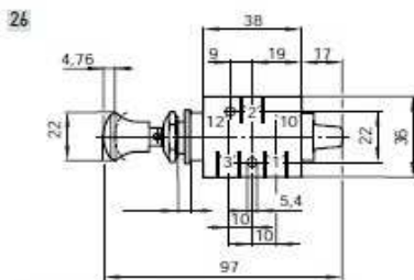
Manopola girevole - G1/8" Rotary knob - G1/8"
