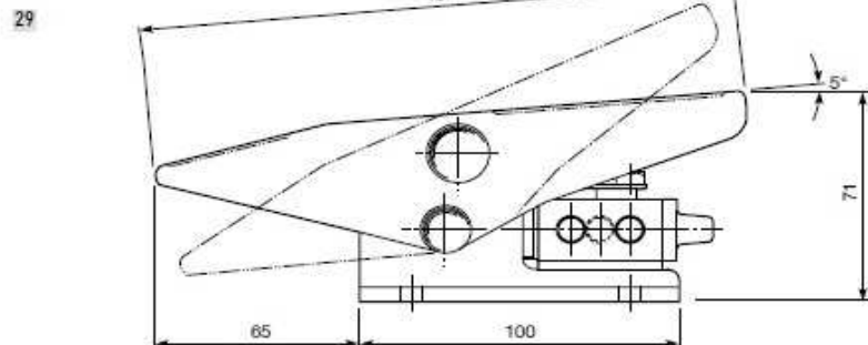
Pedale/Pedal G1/8" - G1/4"
