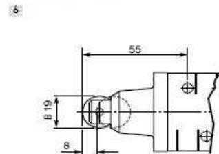
Rullo - valvole G1/4" Roller - G1/4" valves
