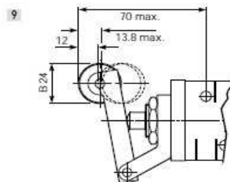
Leva a rulli - valvole G1/4" Roller lever - G1/4" valves
