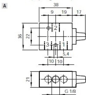
G1/8" - 3/2, ritorno a molla, corpo base G1/8" - 3/2, spring return, basic body
